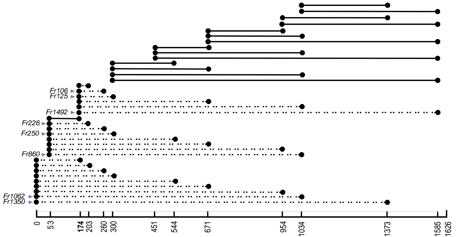
Fig. 3. Schematic of the products amplified with the UMC1651626 -derived STS primers. Primer locations are represented by filled circles. Polymorphic products are represented by dotted lines. Monomorphic products are represented by solid lines. STS markers are identified by blue arrowheads. Primers that originate from opposite sides of the 174-nucleotide position amplify polymorphic products. Primers positioned on the same side result in monomorphic amplifications.
